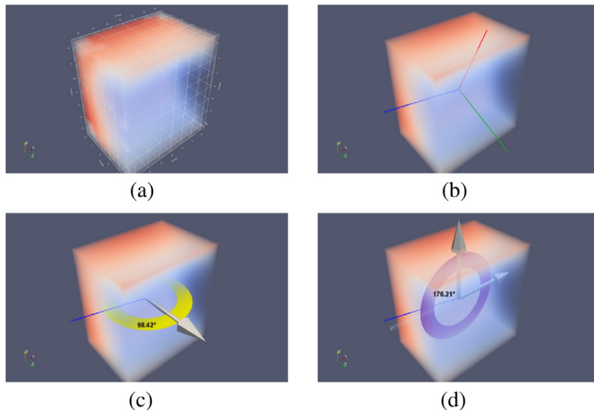
Fig. 10. 4D Nebula feature construction: (a) sample voxel; (b) resulting polynomial volume; principal axes shown in red, green, and blue, in order of curvature magnitude (label = 14, cylinder); (c) \varphi (phi) angle of least curvature direction from the time axis (shown as Z axis in image); (d) \theta (theta) angle of least curvature direction in the XY plane.
